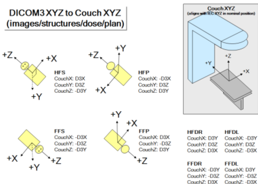
Fig. 4: IEC Coordinate Systems
